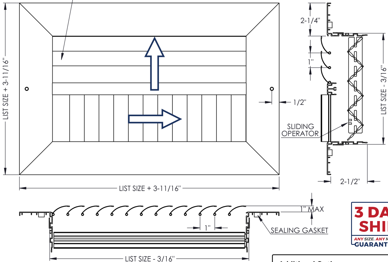
INDIVIDUALLY ADJUSTABLE CURVED BLADES ON 1" SPACING
