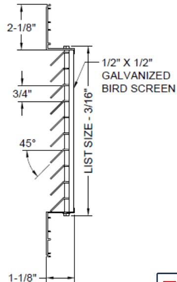
Standard Construction
