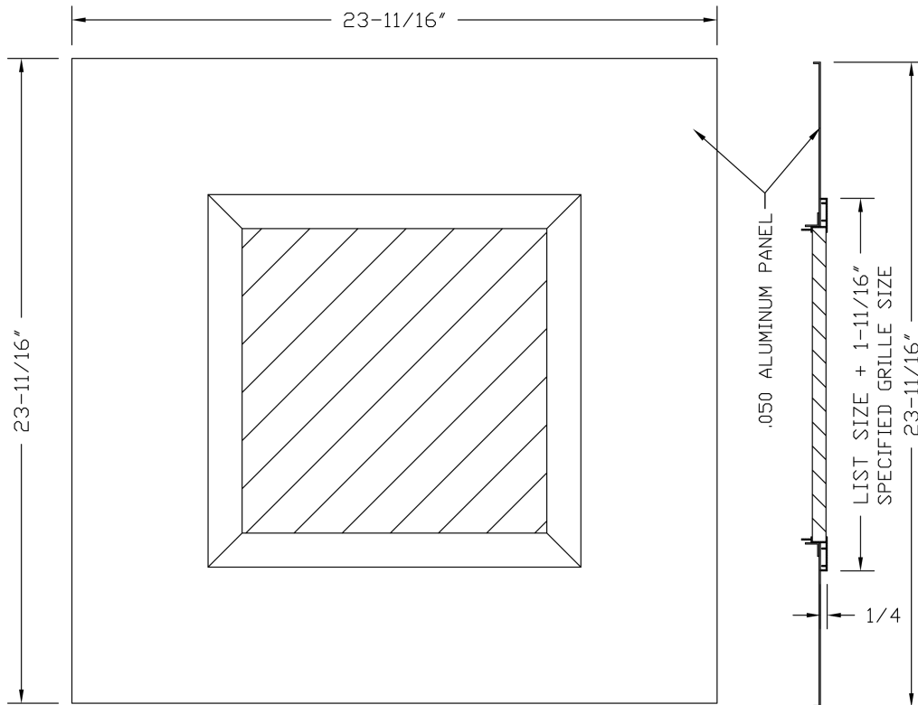
DARE1.1 grille not included (shown as example only)
