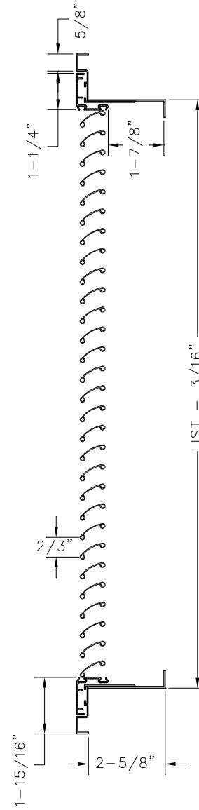
A Spring Pins - Removable Grille (Recommended for Top Mounting Only)
